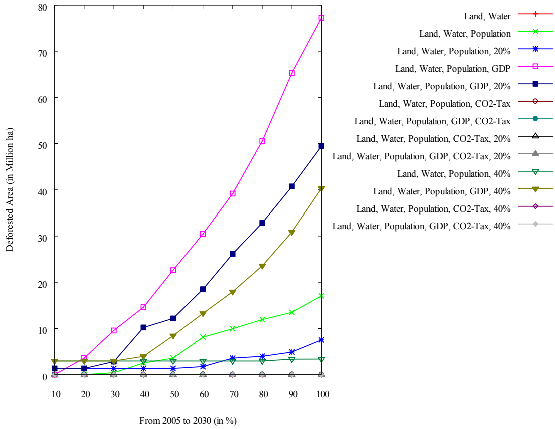
Figure 2 Global deforested area
